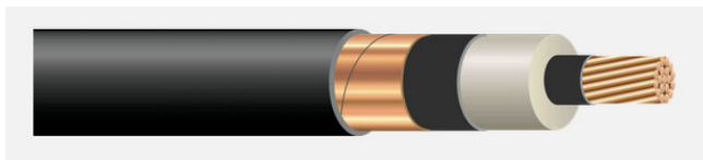
Southwire 35kV Cu NLEPR PVC Medium Voltage Power Cable
